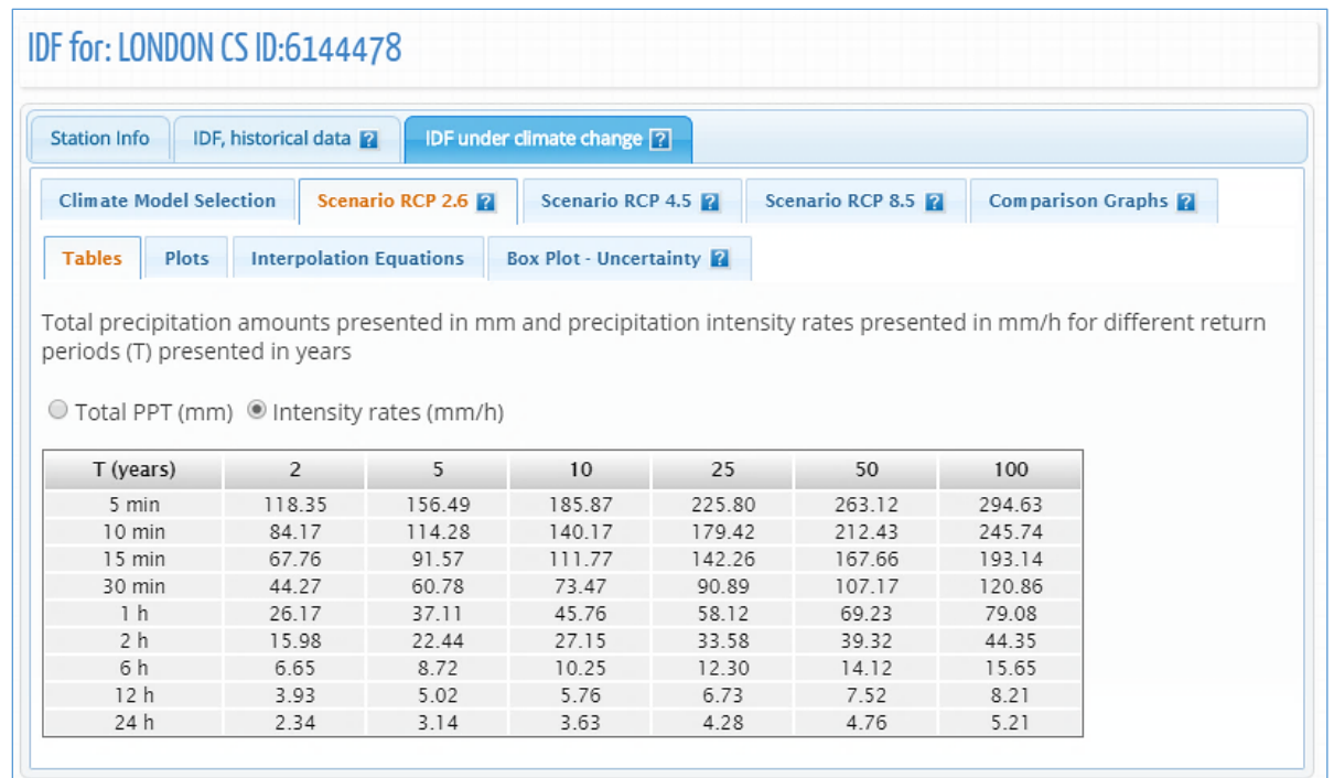
Figure 61. Updated IDF tables for future climate conditions – rainfall intensity in mm/h
