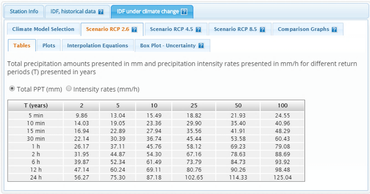
Figure 60. Updated IDF tables for future climate conditions – total precipitation in mm using CMIP5 GCMs
