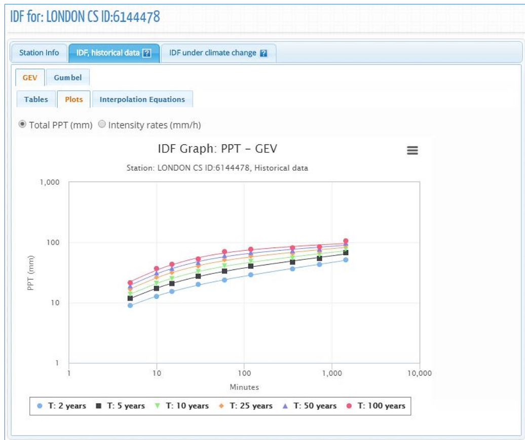
Figure 48. Total precipitation (in mm) IDF graph for different return periods
